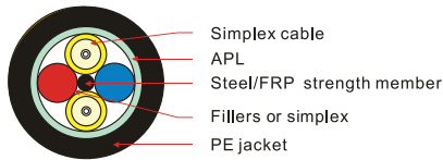
Outdoor/Indoor Cable(2-12F)
