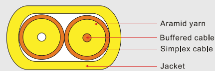
Flat Twin Cable(2F)
