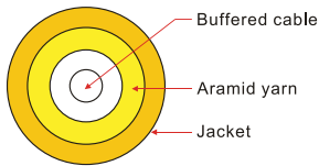
Indoor Simplex Cable(1F)
