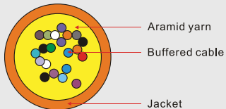
Indoor Distribution Cable(2-48F)
