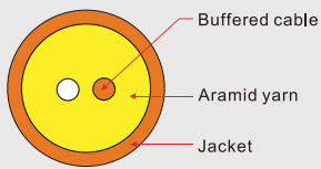
Duplex Round Cable(2F)
