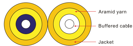
Duplex Zipcord Cable(2F)
