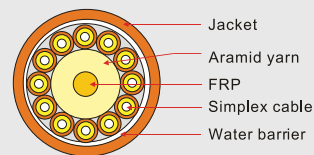
Breakout Cable(2-48F)
